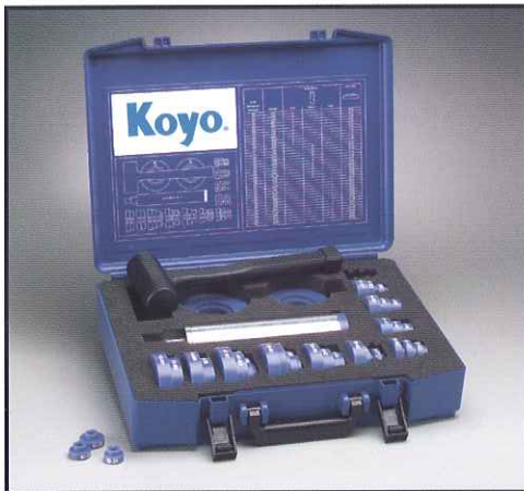
Bearing Mounting Tool Kit BMT33
